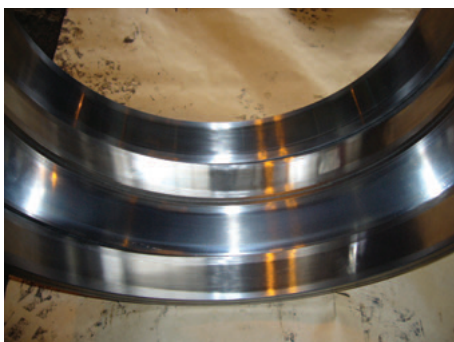
Fig. 8 Post-use appearance of bearing with newly developed steel
