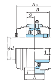
Pressed stainless steel covers
